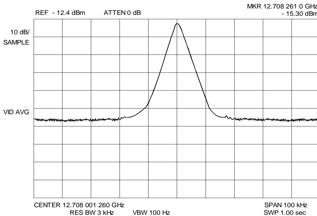
Figure 9-1: Spectrum Analyzer Display during G/T Measurement (Carrier Level)
