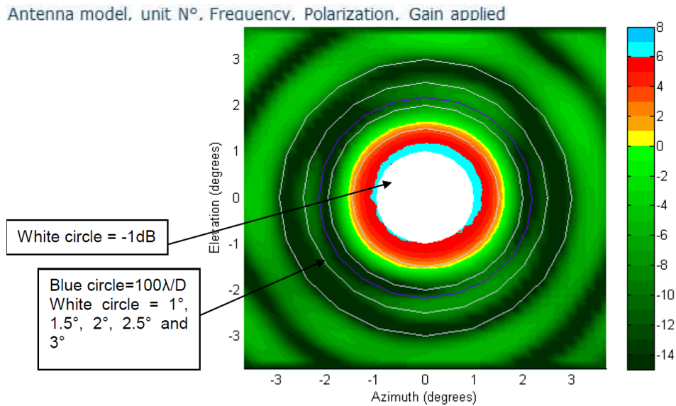
Figure 7-3: co-polar normalized raster scan
