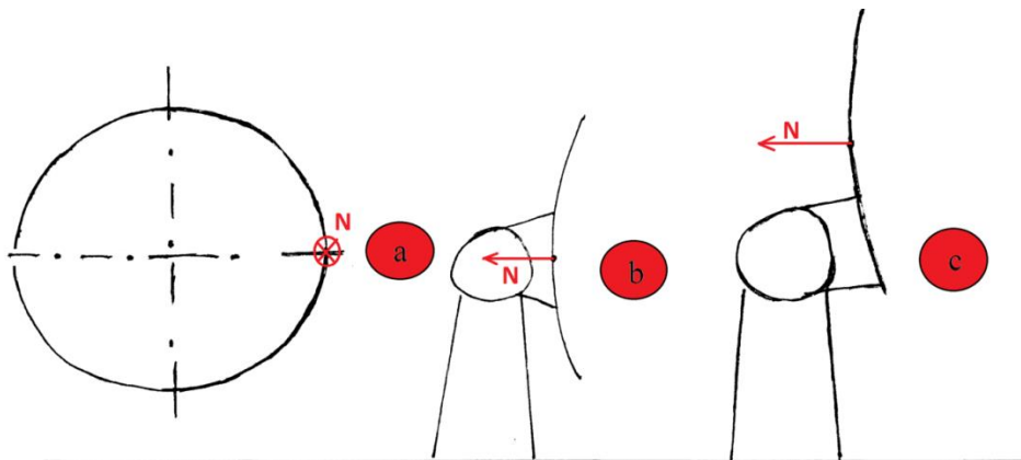
Figure 11-6: Yaw load certification. A) front view of reflector with mounting points for force gauge; b) side view; c) mounting points for offset-mounted antennas.
