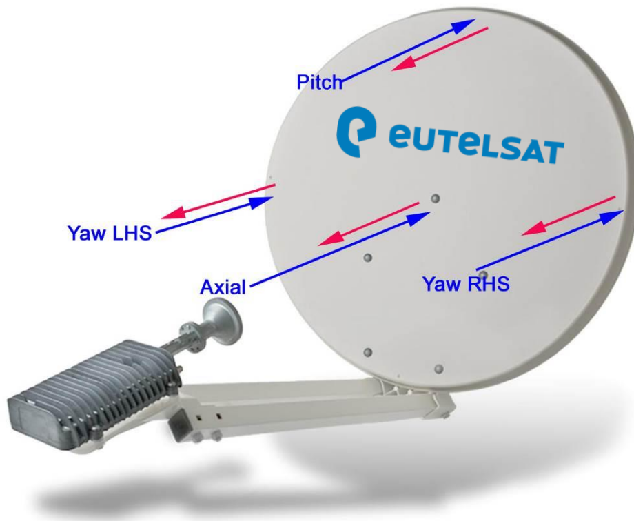
Figure 11-1: Parabolic antenna forces, measured for wind load certification procedure
