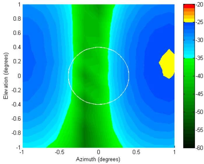
Figure 7-4: cross-polarization normalized raster scan
