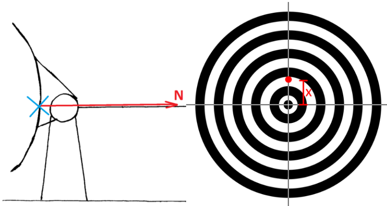
Figure 11-4: Applying the test force N on the antenna under test (left). Example for an ideal offset due to axial load on offset diagram (right)
