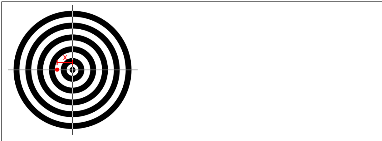
Figure 11-7: Example for an ideal offset due to yaw loads on offset diagram
