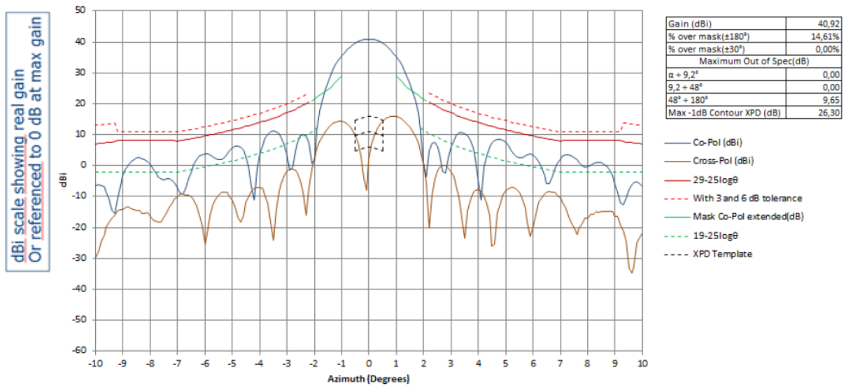
Figure 7-1: example 1 of antenna pattern diagrams
