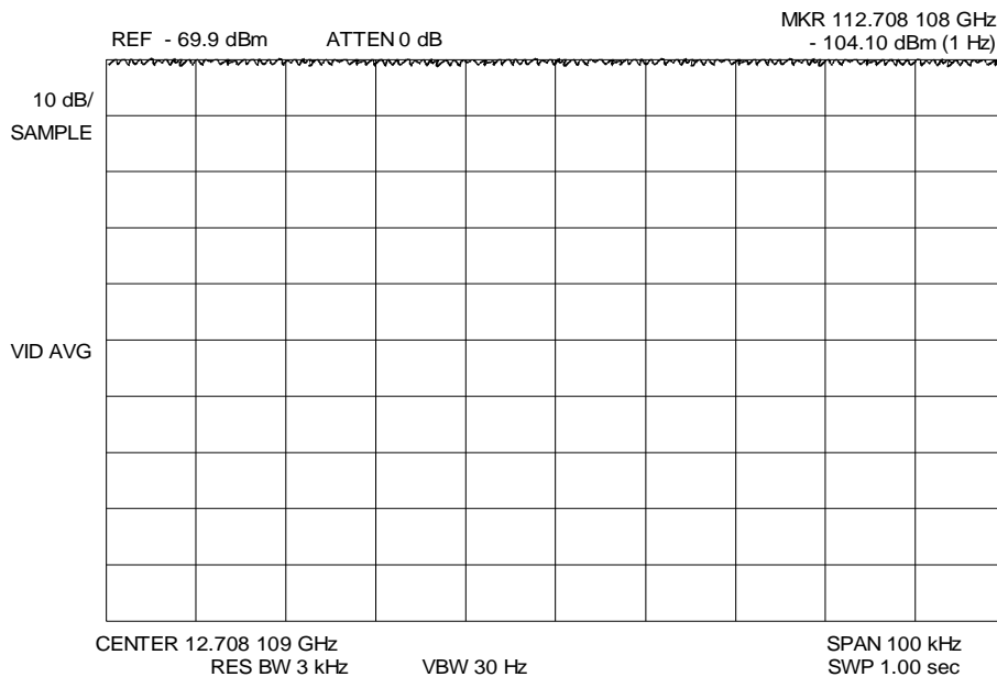
Figure 9-3: Spectrum Analyzer Display during G/T Measurement (Noise Level)
