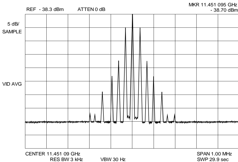
Figure 9-2: Spectrum Analyzer Display during G/T Measurement (Carrier Level)
